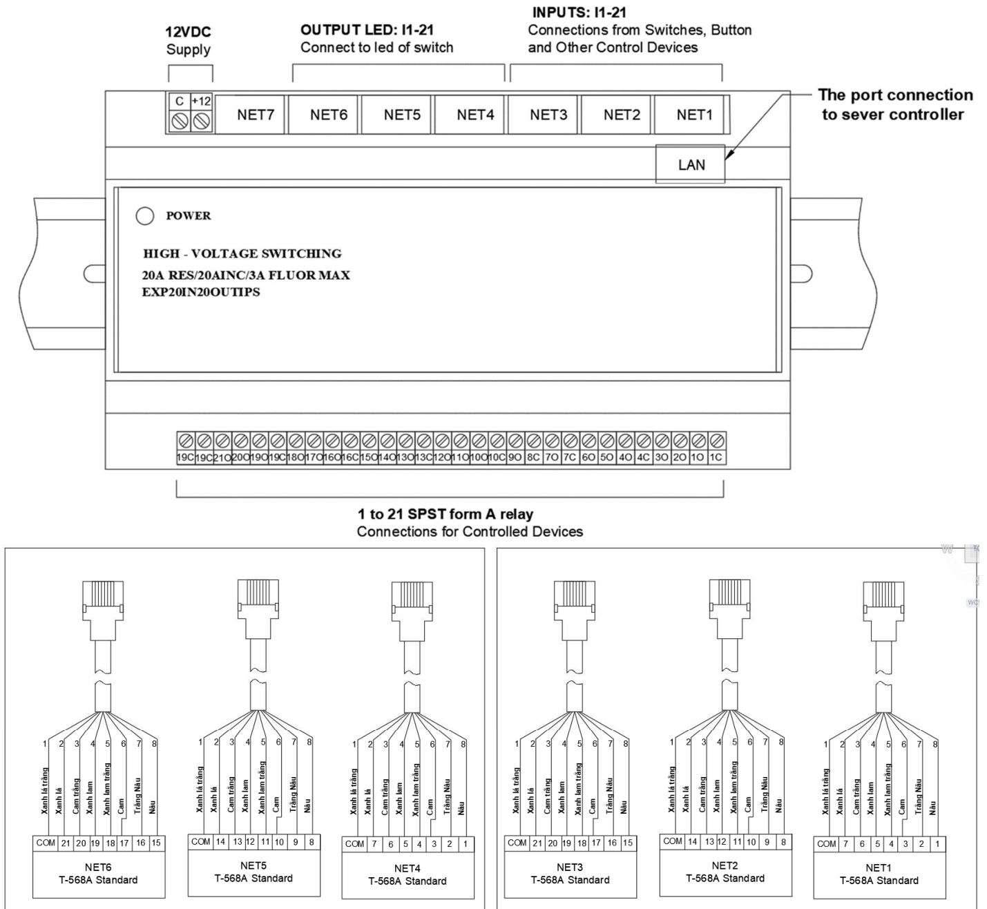
Recommended connection diagram
